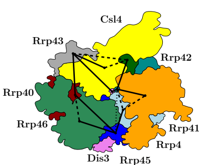
C MILP
