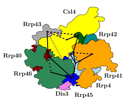
B GREEDY
