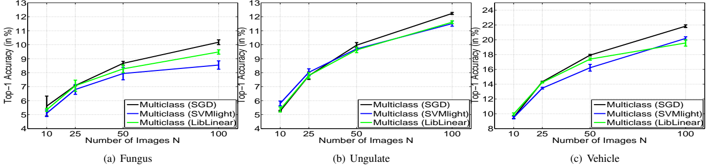
Fig. 2. Comparison of SGD, SVM light and LibLinear for optimizing the MUL SVM using using 4,096-dim BOV. From left to right: Fungus, Ungulate and Vehicle.
