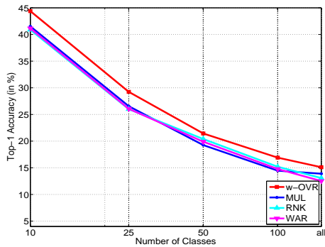
Fig. 7. Top-1 accuracy as a function of the number of classes.
