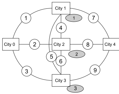
Figure 2: Schematic view, and 3 instances, of MULTIZENO benchmark. Flight durations are attached to the possible routes (white circles), costs/risks are attached to landing in the central cities (grey circles). Three sets of values are given on the right, corresponding to Pareto fronts of Figure 3.
