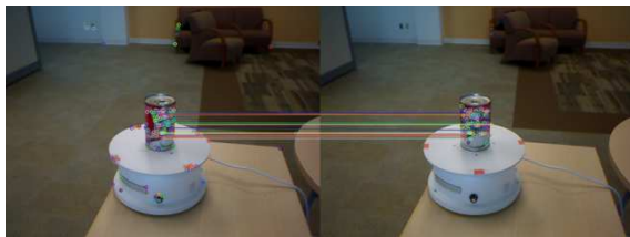
Figure 7: Non-planar object keypoint matching using DARP finds 14 matches.
