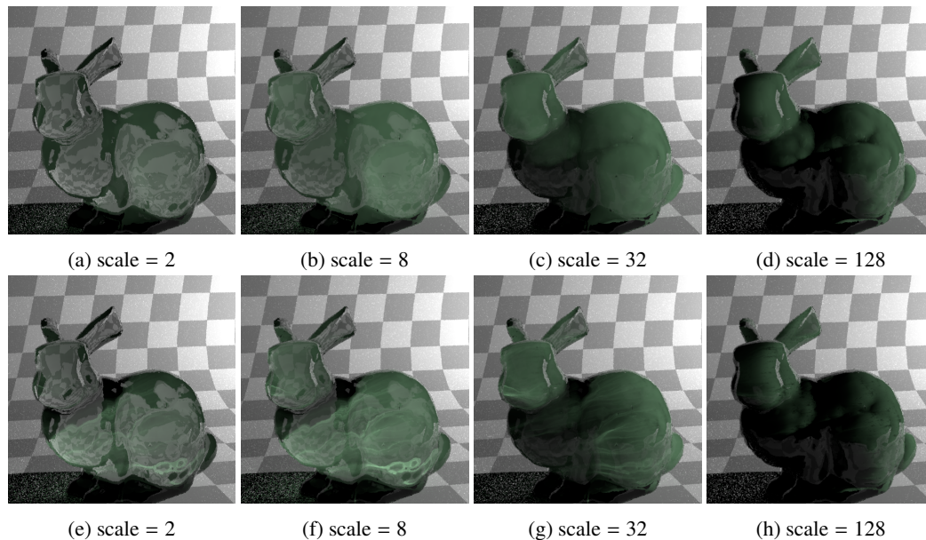
Figure 10: Influence of the scale parameter on single scattering effects. Top row: straight line approximation (10 s). Bottom row: our algorithm (9.46 mn).
