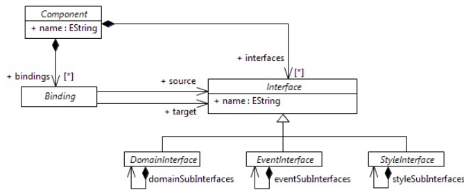
Figure 4: Component Metamodel
