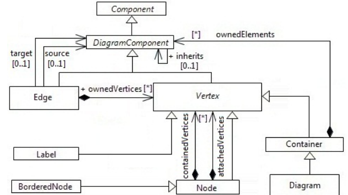
Figure 5: Diagram Elements
