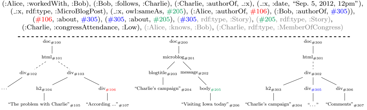
Fig. 1: XR instance representing annotated documents.
