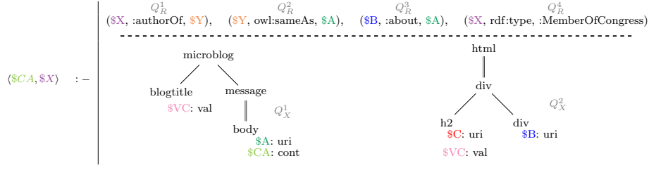
Fig. 2: Sample XRQ query
