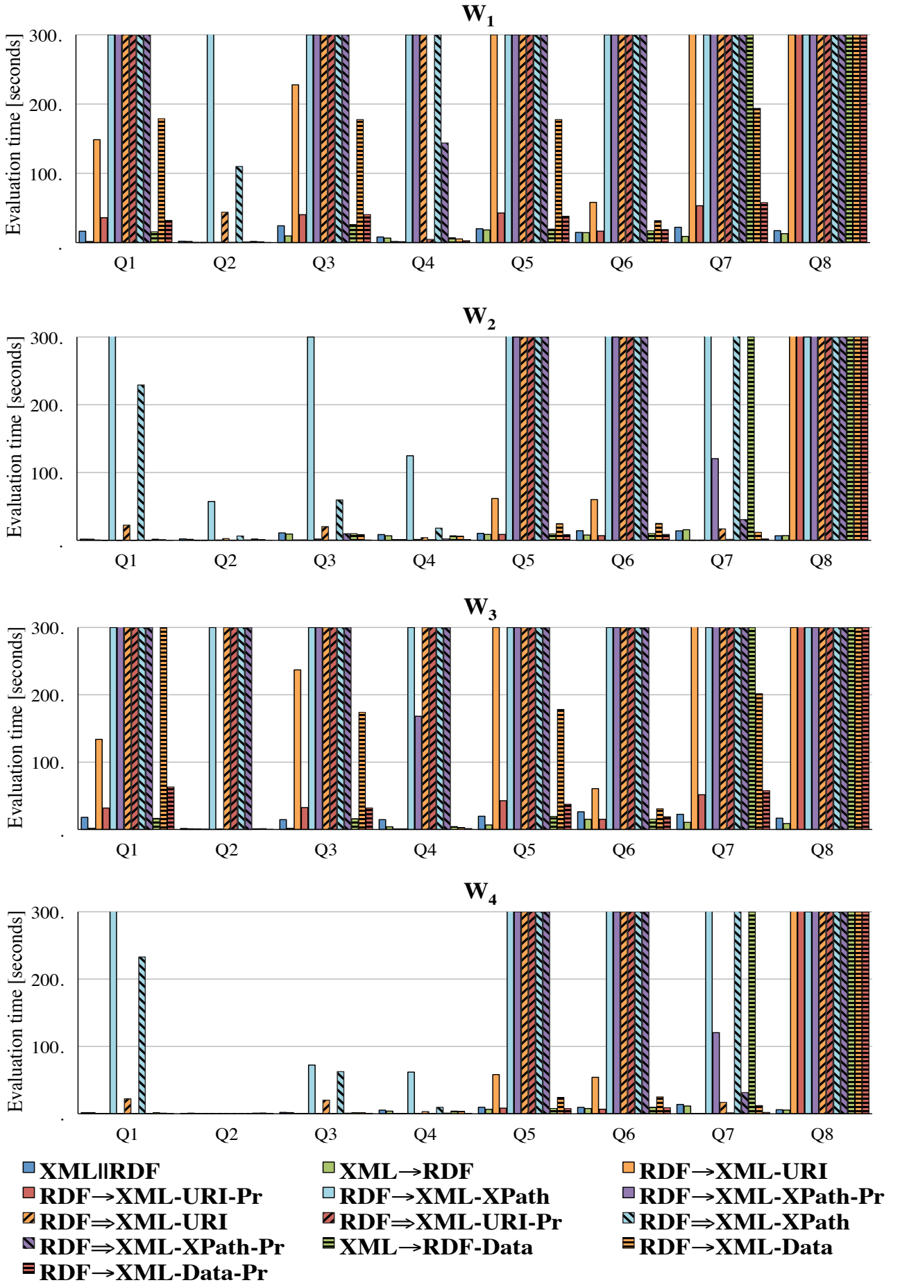
Fig. 7: XR query evaluation strategies compared on workloads W_1 - W_4 and dataset \mathcal{D}_1^1 .
