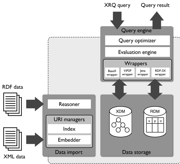
Fig. 6: Architecture of the XR platform.
