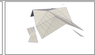
Fig. 15 Reconstruction of an aerial LIDAR point cloud capturing the rooftop of a house. Top: input point set, middle: final reconstruction, bottom: two other views. The reconstruction yields a very simplified mesh despite the noise. Point set courtesy of Qian-Yi Zhou and Ulrich Neumann.
