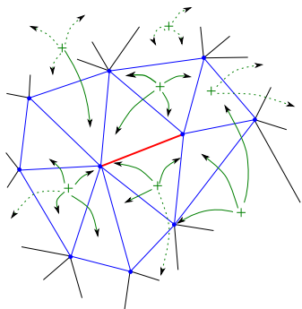
Fig. 5 Local stencil of an edge. For better depiction we represent a manifold neighborhood of an edge (in red) and do not depict the bins. Simplices in the local stencil are depicted in blue. Point samples are depicted in green. We only solve for the measures transported to the stencil (solid green lines) and not for the measures transported outside of the stencil (dash green lines).
