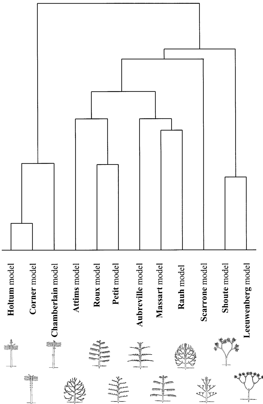
Figure 9. Taxonomy tree whose terminal vertices correspond to architectural models and the non-terminal vertices represent the distances between the models appearing on the leaves.
