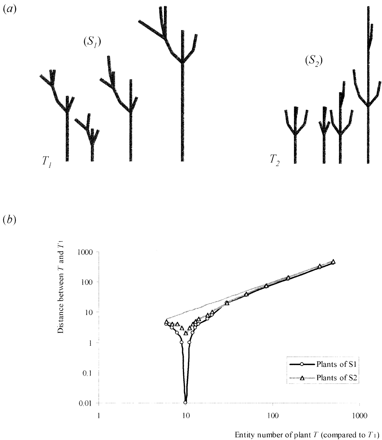
Figure 6. Topological comparison. (a) Sets S_1 and S_2 of theoretical plants built from T_1 and T_2 . (b) Distance from plants of S_1 and S_2 to reference plant T_1 on a logarithmic scale.
