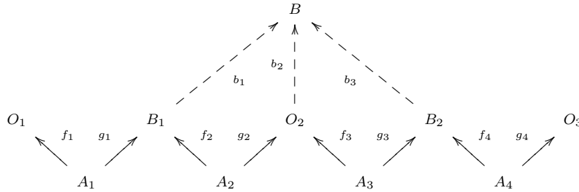
Figure 4. Composing W-alignments.
