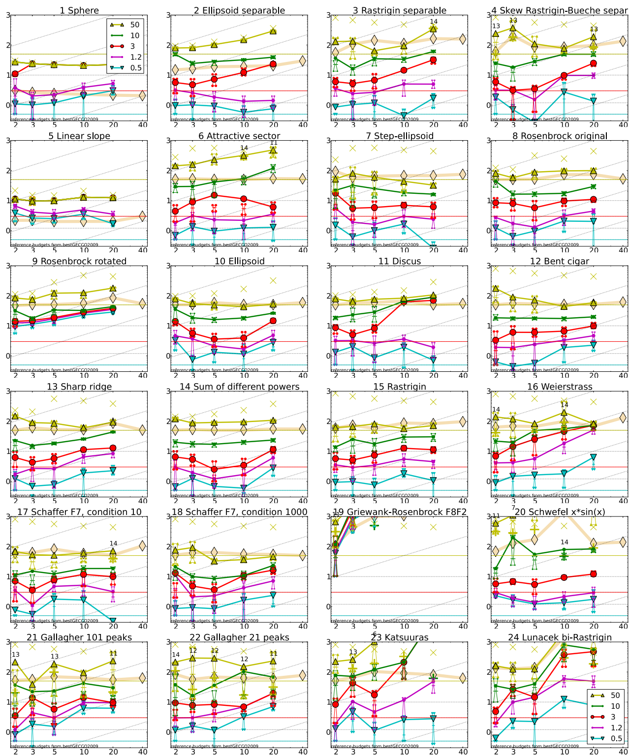
Figure 2: Expected number of f -evaluations (ERT, lines) to reach f_{\text{opt}} + \Delta f ; median number of f -evaluations (+) to reach the most difficult target that was reached not always but at least once; maximum number of f -evaluations in any trial ( \times ); interquartile range with median (notched boxes) of simulated runlengths to reach f_{\text{opt}} + \Delta f ; all values are divided by dimension and plotted as \log_{10} values versus dimension. Shown is the ERT for targets just not reached by the artificial GECCO-BBOB-2009 best algorithm within the given budget k \times \text{DIM} , where k is shown in the legend. Numbers above ERT-symbols indicate the number of trials reaching the respective target. The light thick line with diamonds indicates the respective best result from BBOB-2009 for the most difficult target. Slanted grid lines indicate a scaling with \mathcal{O}(\text{DIM}) compared to \mathcal{O}(1) when using the respective 2009 best algorithm.
