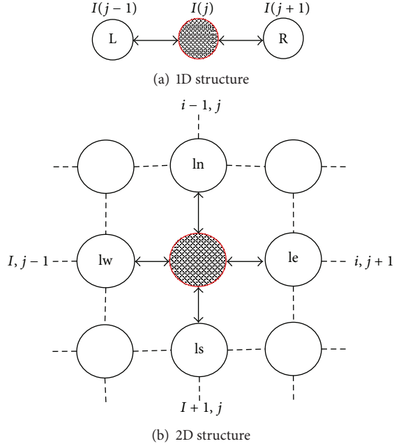
FIGURE 3: Gradient computation. (a) One-dimensional (1D) grid structure: the signal flow is calculated between two neighboring nodes (solid connection). (b) Two-dimensional (2D) grid structure: the signal flow is calculated between four neighboring nodes (solid connection).
