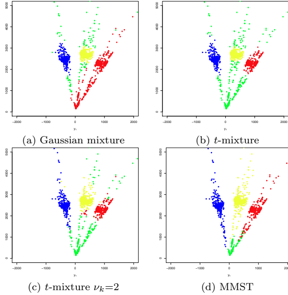
Fig. 4 Classification results with K = 4 for the audiovisual recording data. Classifications are shown in the first (x-axis) and third (y-axis) dimensions for (a) a Gaussian, (b) standard t , (c) standard t with all \nu_k = 2 mixtures and (d) for the MMST. The different colors indicate the 4 different components to which observations are assigned to.
