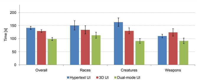
Figure 13: Overall results.
