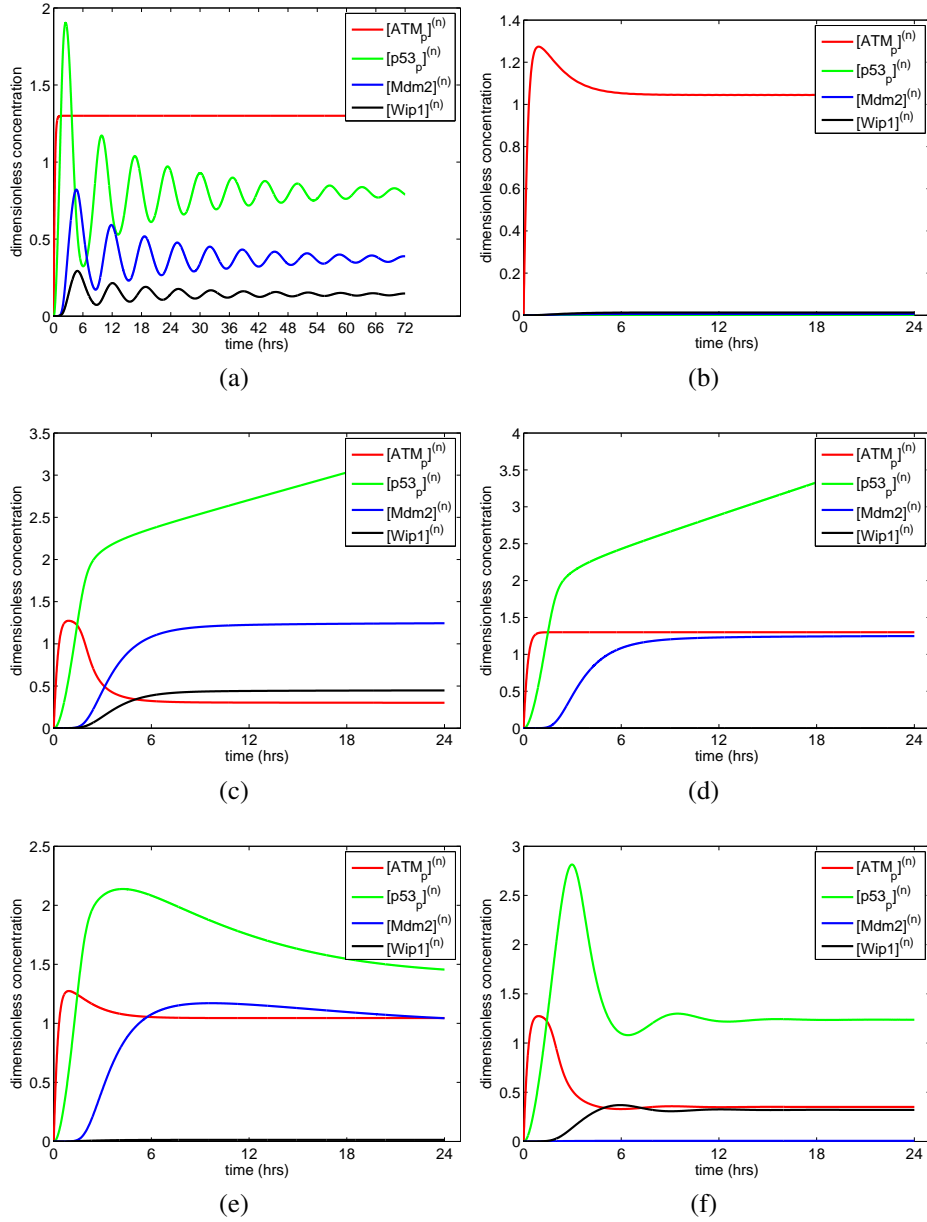
Figure D.3: (a) Inhibition of the negative feedback Wip1 \dashv ATM , k_{dph2} = 0 in (4). (b) Inhibition of the positive feedback ATM \rightarrow p53 , k_3 = 0 in (6) (c) Inhibition of the negative feedback Wip1 \dashv p53_p , k_{dph1} = 0 in (6). (d) Inhibition of the positive feedback p53_p \rightarrow Wip1 , k_{S_{pw}} = 0 and k_{S_w} = 0 (the basal production rate). (e) Inhibition of the positive feedback p53_p \rightarrow Wip1 , k_{S_{pw}} = 0 and k_{S_w} = 0.03 (the basal production rate). (f) Inhibition of the positive feedback p53_p \rightarrow Mdm2 , k_{S_{pm}} = 0 and k_{S_m} = 0.005 (the basal production rate).
