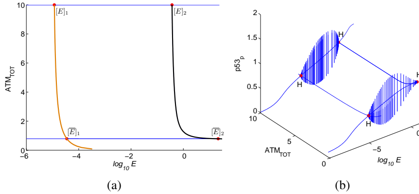
Figure 4.9: (a) The evolution curves of both Hopf bifurcation points (curves in brown and black colours). The Hopf bifurcation points [E]_1 and [E]_2 are computed for ATM_{TOT} = 10\mu M , the points [\bar{E}]_1 and [\bar{E}]_2 for ATM_{TOT} = 0.78\mu M . The concentration E = [E] is in the logarithmic scale. (b) Bifurcation diagrams of p53_p with respect to changing ATM_{TOT} and [E] .
