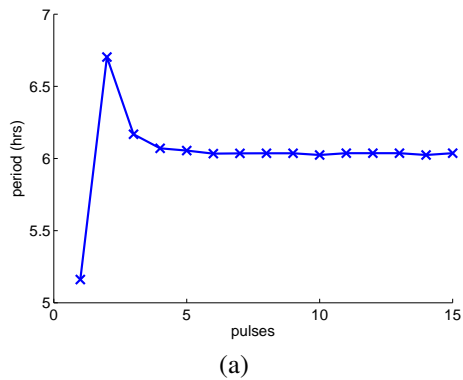
Figure D.2: (a) The periods of the fifteen p53_p pulses produced by the ODE model within [E] = 0.1 . The length of the first pulse is 5.16 hours, the p53_p stable limit cycle is of the period \sim 6 hours.
