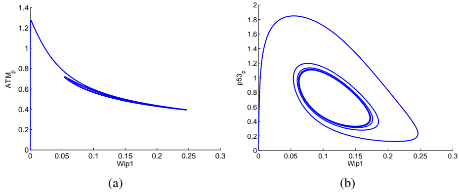
Figure D.1: Phase planes relative to the involved nuclear proteins within [E] = 0.1\mu M (a) Wip1 and ATM_p (b) Wip1 and p53_p .
