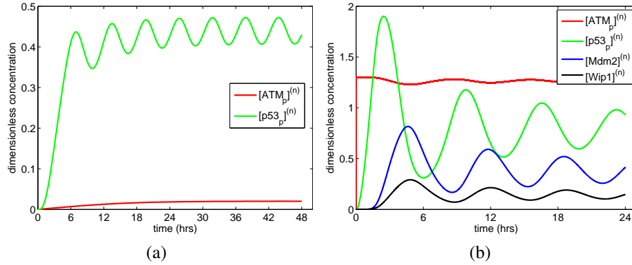
Figure 4.6: (a) Nuclear p53_p/ATM_p concentrations from the ODE system for [E] = [E]_1 = 2.5 \times 10^{-5} \mu M . The concentration of ATM_p converges to the equilibrium point and the concentration of p53_p tends to a stable limit cycle. (b) Nuclear ATM_p/p53_p/Mdm2/Wip1 concentrations for [E] = 10 \mu M . The concentration of ATM_p is of small amplitude, getting even smaller with further increasing [E] . Plotted concentrations are dimensionless, ATM_{TOT}(0) = 1.3 \mu M .
