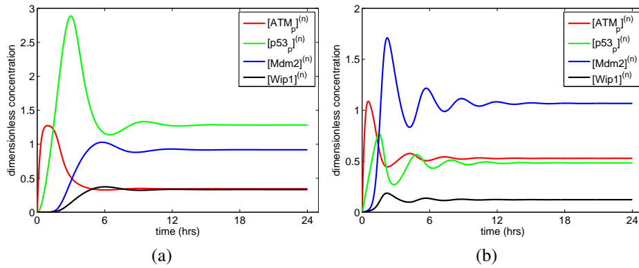
Figure 4.8: (a) The ATM/p53/Mdm2/Wip1 dynamics over a 24 hour-long time interval, [E] = 0.1\mu M , in a case when Mdm2-mediated ubiquitination of p53 is inhibited, k_1 = 0 . (b) The ATM/p53/Mdm2/Wip1 dynamics over a 24 hour-long time interval and [E] = 0.1\mu M in a case when only one compartment is considered.
