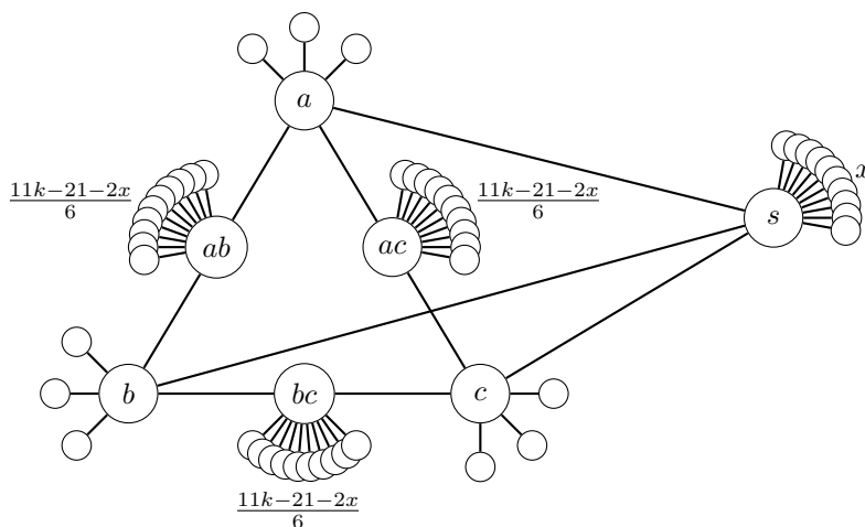
Figure 2: Scheme of the graph family described in the proof of Theorem 7.
