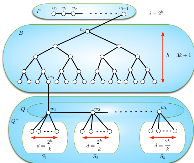
Figure 3: Tree T_k described in the proof of Theorem 8.
