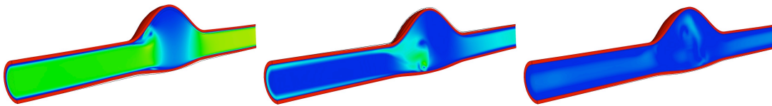
Figure 12: Snapshots of the fluid velocity and solid deformation at t = 0.2016, 0.336, 0.672 (from left to right). The solid line represents the reference configuration of the solid.
