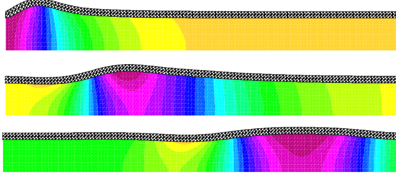
Figure 3: Snapshots of the fluid pressure and solid displacement at t = 0.003, 0.008, 0.015 (from top to bottom). Algorithm 2 with second-order extrapolation and first-order correction, \gamma_0 = 1 , \gamma = 1000 , \tau = 10^{-4} and h = 0.05 .
