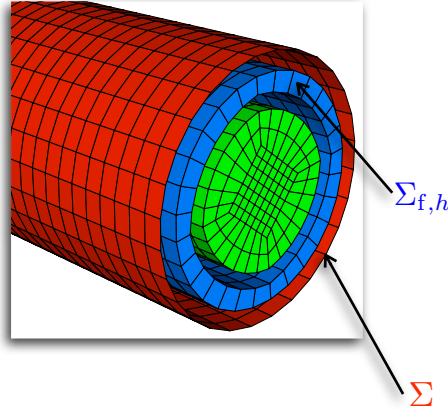
Figure 2: The fluid layer of elements, \Sigma_{f,h} , adjacent to the fluid-solid interface \Sigma .
