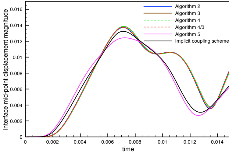
Figure 9: Comparison of the implicit, the Robin-Robin explicit coupling schemes without second-order extrapolation and Algorithm 5: interface mid-point displacement magnitude vs. time.
