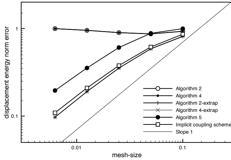
Figure 5: Solid displacement error convergence histories (in the relative elastic energy-norm) at time t = 0.015 with \tau = \mathcal{O}(h) .
