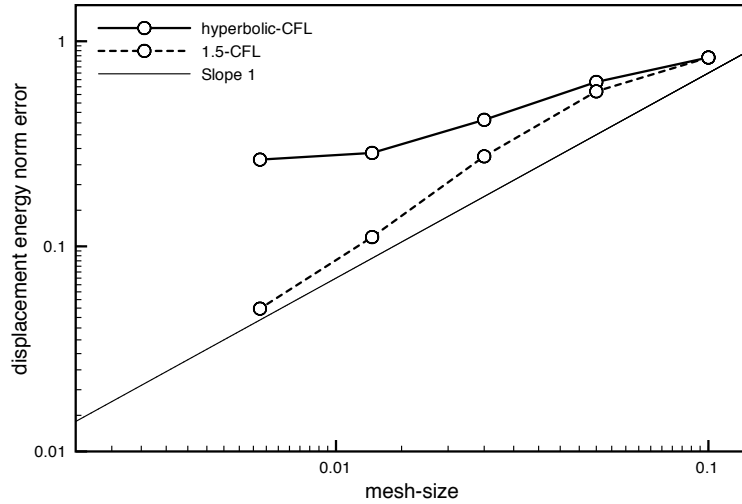
Figure 4: Solid displacement error convergence histories (in the relative elastic energy-norm) at time t = 0.015 , obtained from Algorithm 2 with one correction, for \gamma_0 = 1 , \gamma = 1000 , \tau = \mathcal{O}(h) (hyperbolic-CFL) and \tau = \mathcal{O}(h^{\frac{3}{2}}) (1.5-CFL).
