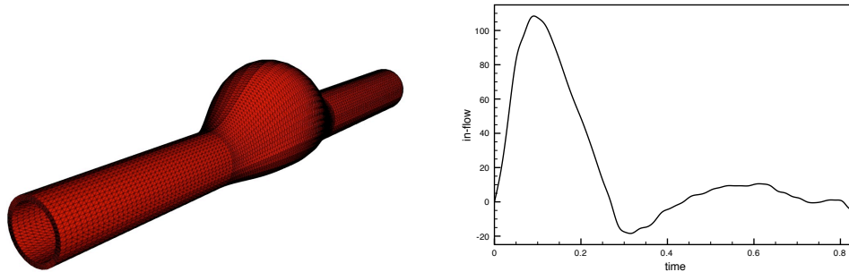
Figure 11: Aneurysm geometry (left) and in-flow rate data (right).
