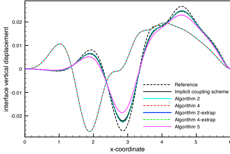
Figure 7: Comparison of the interface displacement at time t = 0.015 obtained with (\tau, h) = (5 \times 10^{-4}, 10^{-1})/16 .
