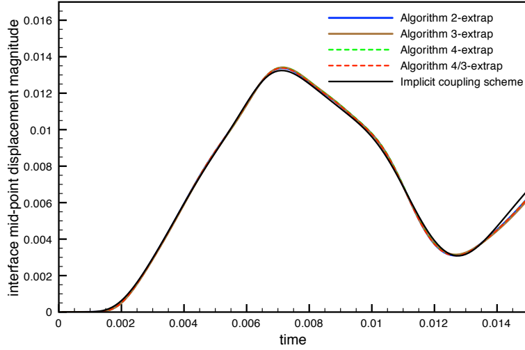
Figure 10: Comparison of the implicit and Robin-Robin explicit coupling schemes with second-order extrapolation: interface mid-point displacement magnitude vs. time.
