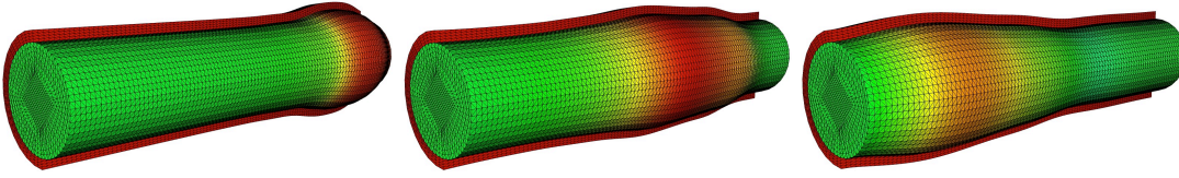
Figure 8: Snapshots of the fluid pressure and solid deformation at t = 0.003, 0.007, 0.011 (from left to right) obtained with Algorithm 3 ( \gamma_0 = 1, \gamma = 2500 ) with the second-order extrapolation and the first-order correction.
