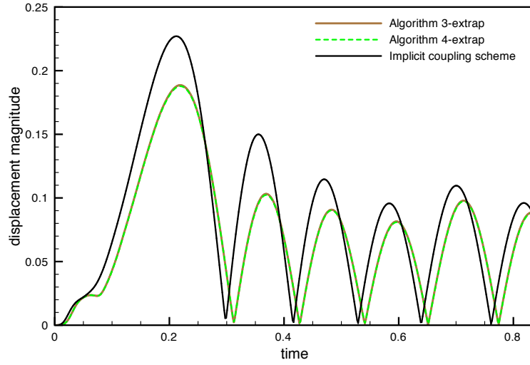
Figure 14: Comparison of the implicit and Robin-Robin explicit coupling schemes with second-order extrapolation: interface mid-point displacement magnitude vs. time.
