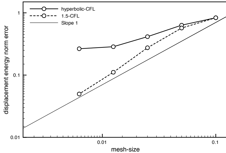
Figure 4: Solid displacement error convergence histories (in the relative elastic energy-norm) at time t = 0.015 , obtained from Algorithm 2 with and the first-order correction, for \gamma_0 = 1 , \gamma = 1000 , \tau = \mathcal{O}(h) (hyperbolic-CFL) and \tau = \mathcal{O}(h^{\frac{3}{2}}) (1.5-CFL).
