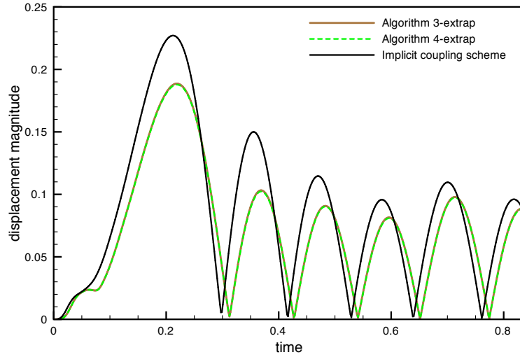
Figure 14: Comparison of the implicit and Robin-Robin explicit coupling schemes with second-order extrapolation: interface mid-point displacement magnitude vs. time.
