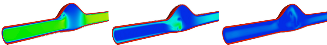
Figure 12: Snapshots of the fluid velocity and solid deformation at t = 0.2016, 0.336, 0.672 (from left to right). The solid line represents the reference configuration of the solid.
