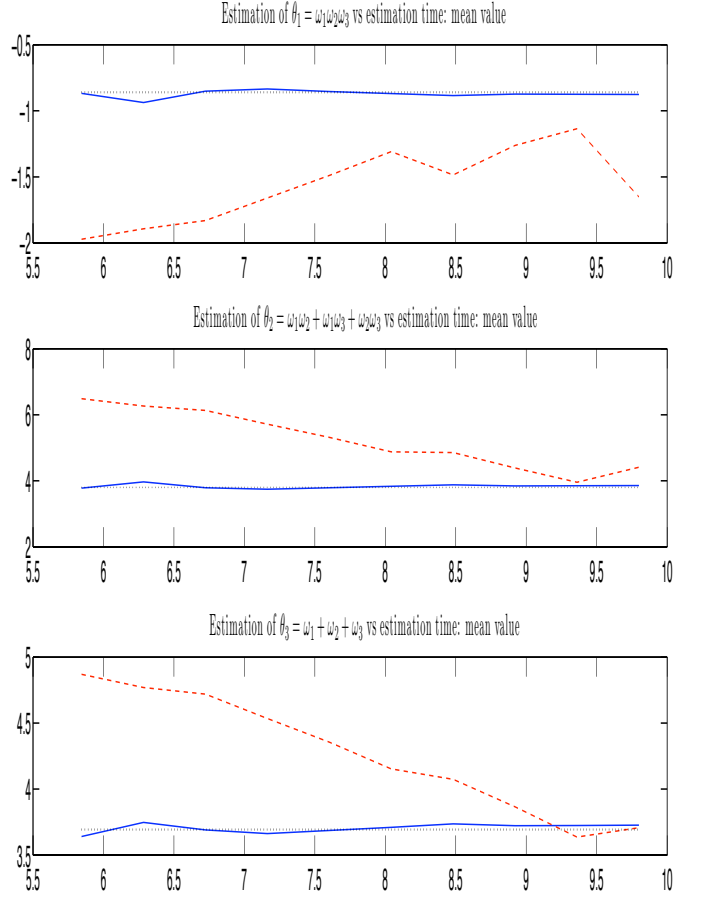
Fig. 1. Comparison with the modified Prony’s method
