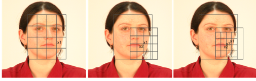
Figure 2: Three successive steps of regression for the Left Mouth Corner
