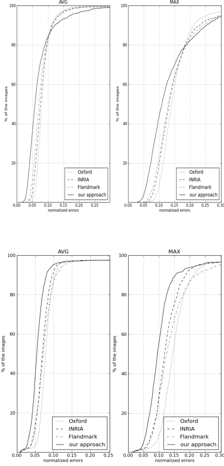
Figure 5: Cumulative distribution of point to point error measure on the PUT and MUCT test set.
