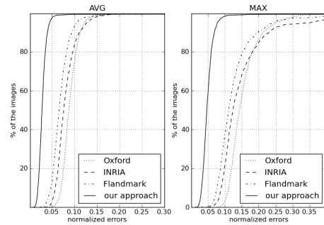
Figure 4: Cumulative distribution of point to point error measure on the BioID test set.
