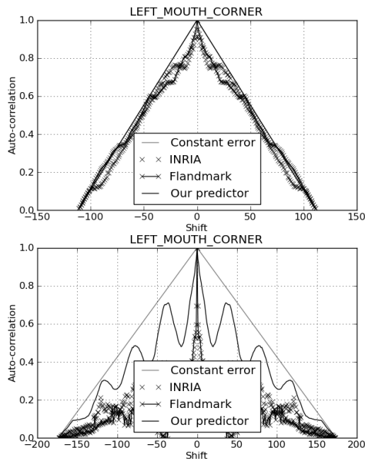
Figure 6: Auto-correlation of the normalized error vector of a non-speaking video sequence (upper graph) and a speaking one (lower graph).
