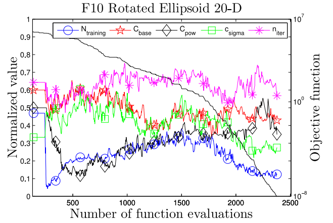
Figure 3: The median trajectories of normalized surrogate hyper-parameters estimated on 15 runs of the original (Left) and modified (Right) versions of IPOP- s* aACM-ES on 20-dimensional Rotated Ellipsoid.
