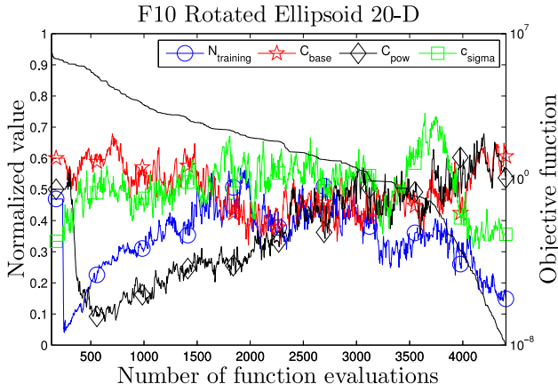
Figure 3: The median trajectories of normalized surrogate hyper-parameters estimated on 15 runs of the original (Left) and modified (Right) versions of IPOP- s* aACM-ES on 20-dimensional Rotated Ellipsoid.
