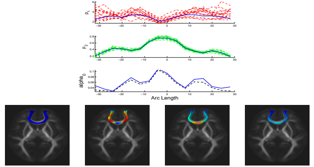
Fig. 5. Top: Estimated normative model parameters (blue) versus individual parameters (red). Bottom: Estimated normative parameters visualized in the coordinate space of genu tract. Left to right: (\alpha_0(s), p_1(s), p_2(s), f_t(s)) at-birth. Color scale is red (high) to blue (low).
