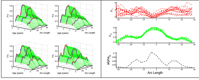
Fig. 3. Application to pediatric data (15 subjects, 3 timepoints): Left: Estimated trajectories for 4 of the 15 subjects (refer to Fig 2 for color codes). Right: Estimated (p_1^B(s), p_2^B(s), \alpha_0(s))
