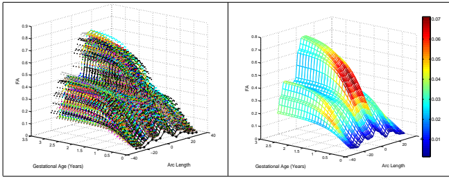
Fig. 4. Normative trajectory: Left: Individual (dots) versus normative (black lines) trajectory. Right: Normative trajectory colored by population standard deviation.
