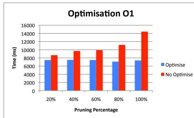
Fig. 33. Performance for reduction rule O1.
