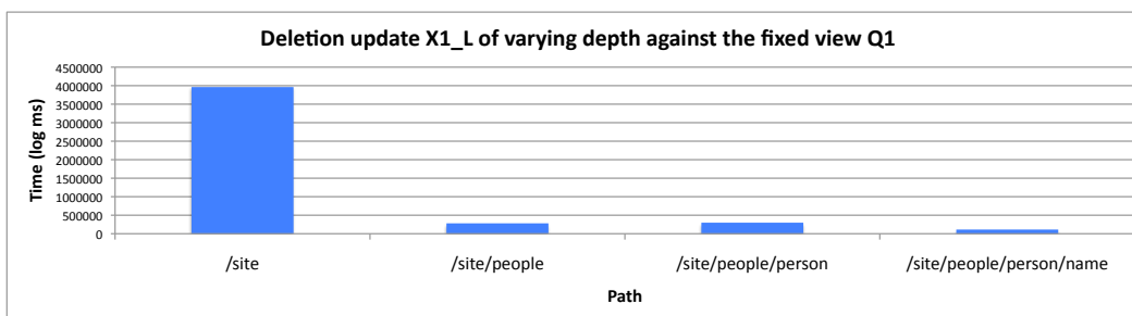
Fig. 23. Varying Paths for XMark view Q_1 and update X1.L on a 10MB database.
