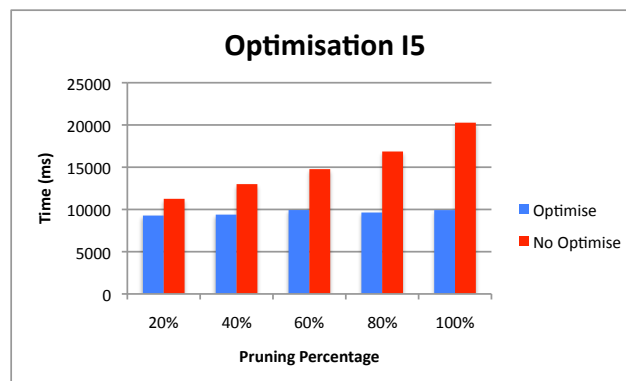
Fig. 35. Performance for reduction rule I5.
