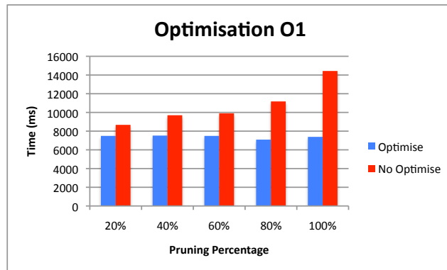
Fig. 33. Performance for reduction rule O1.
