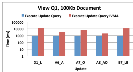
Fig. 28. PINT/PIMT algorithms compared with the IVMA algorithm [Sawires et al. 2005] for view Q_1 .
