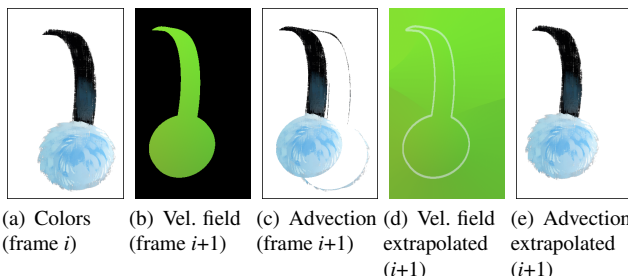
Figure 10: Advection of colors (a) using a standard velocity field (b) can leave overpainted regions behind (c). Our approach extrapolates the velocity field into the background of each layer (d, original outline in white), allowing advection outside the borders of the shape (e).
