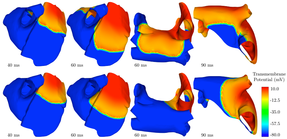
Fig. 4. Simulations of atrial depolarization for homogeneous case i.e. \theta = 0 (top) and for homogeneous and isotropic case (bottom)
