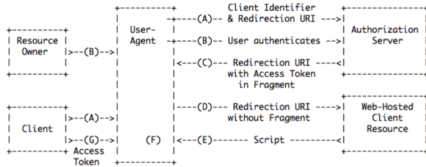
Figure 3: OAuth 2.0: User-Agent Flow.
