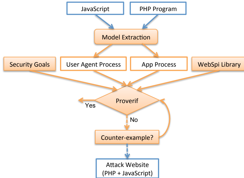
Figure 6: Model extraction and verification framework
