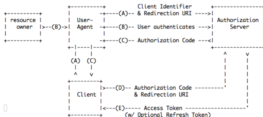
Figure 4: OAuth 2.0: Authorization Code Flow.
