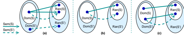
Fig. 3. Valid (a) and invalid (b, c) refinements.
