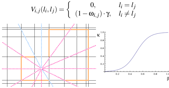
Figure 3: Left: Schematic view of the ray-casting to predict the empty or occupied label for a cell. The cell decomposition is depicted in black and edges with \omega_{i,j} > \frac{1}{2} are depicted in orange. Rays indicating empty, i.e., odd number of intersections, are depicted in pink versus blue. Right: Mapping sigmoid function turning the ratio \kappa of rays indicating empty space to total number of rays into \beta .
