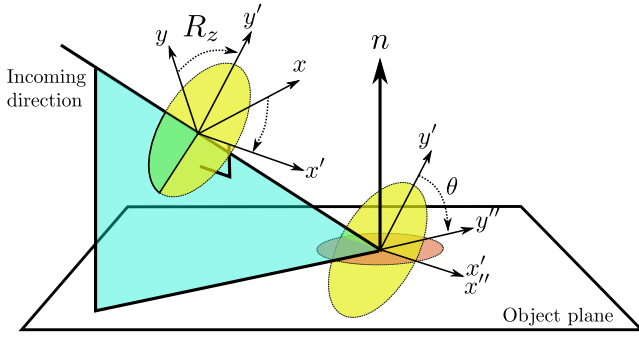
Fig. 5: Successive transformations to convert the incoming light field (with axes x, y ), into the frame of the object (with axes x', y'' ): a rotation R_z to align x with the object's plane and a scale along y' by \frac{1}{\cos \theta} .
