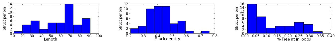
Fig. 4: Number of secondary structures per bin, according to our three clustering criteria.
