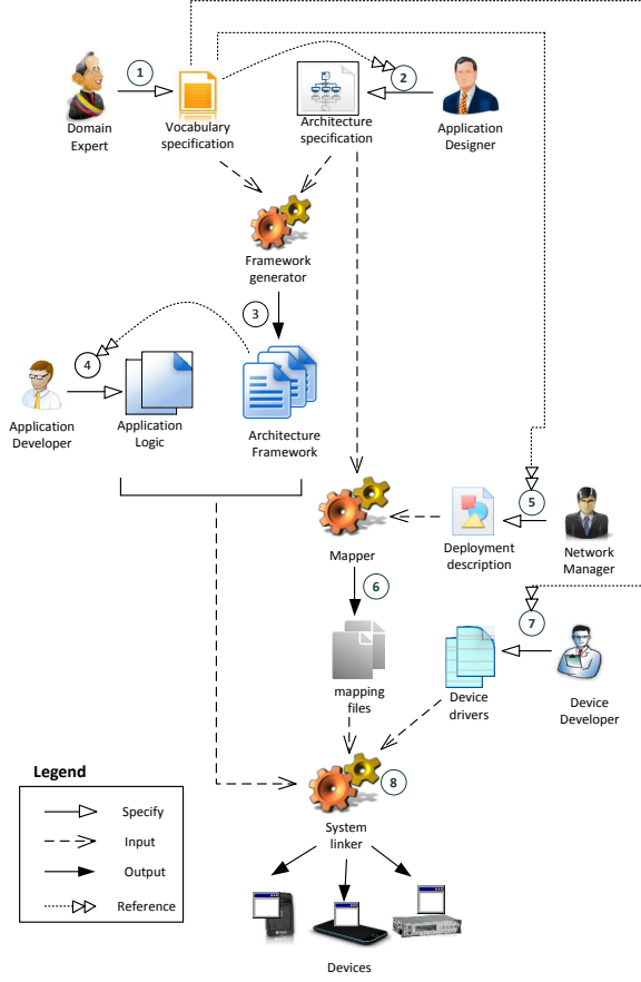
Fig. 2. IoT Application Development using Our Approach
