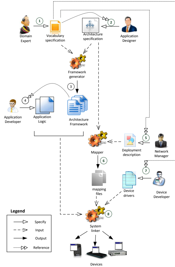
Fig. 2. IoT Application Development using Our Approach
