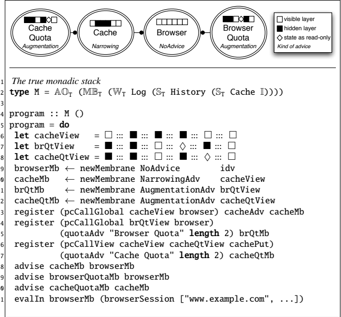
Figure 4: Membrane topology of the composed program. A membrane can only contain aspects that conform to its view and its control flow combinator (adapted from [14]).
