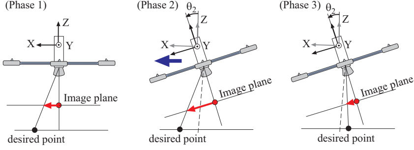
Fig. 5: Effect of Image errors for translational motion in horizontal plane. Positive feedback of the image errors inclines the UAV and generates the translational force in the horizontal direction. As a result, the image errors are eliminated by moving on the left.
