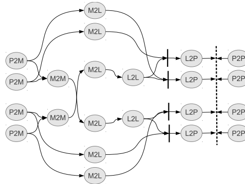
Figure 6: The task flow of the FMM algorithm given by a DAG where nodes represent tasks and edges dependencies (straight lines represent a writing operation from different tasks on the same memory).
