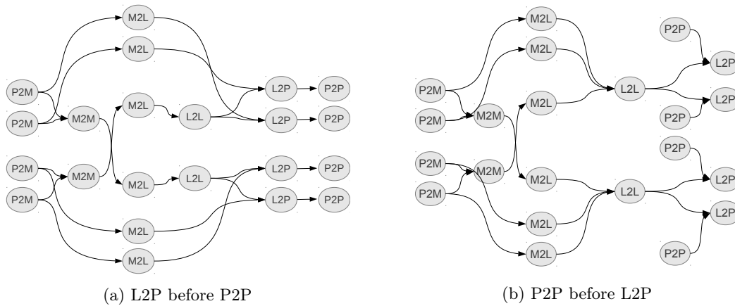
Figure 7: DAG generated by the two P2P and L2P tasks insertion algorithms.
