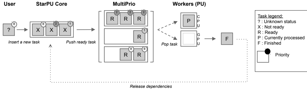
Figure 10: Priority scheduler
