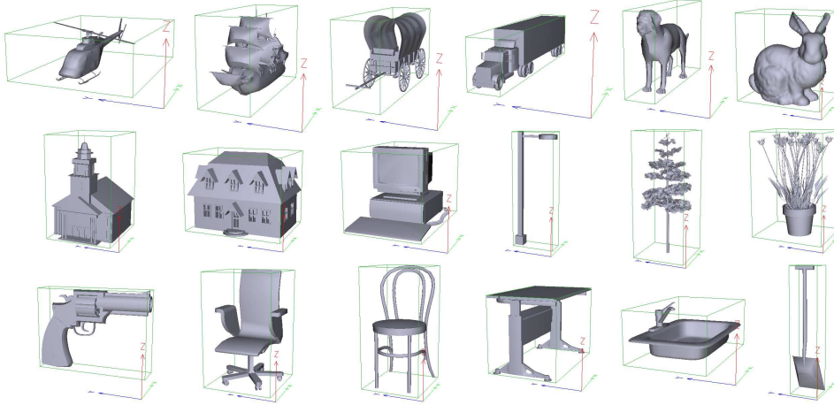
Fig. 6. Alignments of models from different classes using our method.
