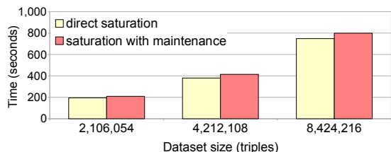
Figure 14: Scalability of our saturation algorithms.
