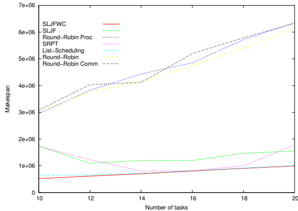
Figure 6. Makespan on a platform with homogeneous slaves.
