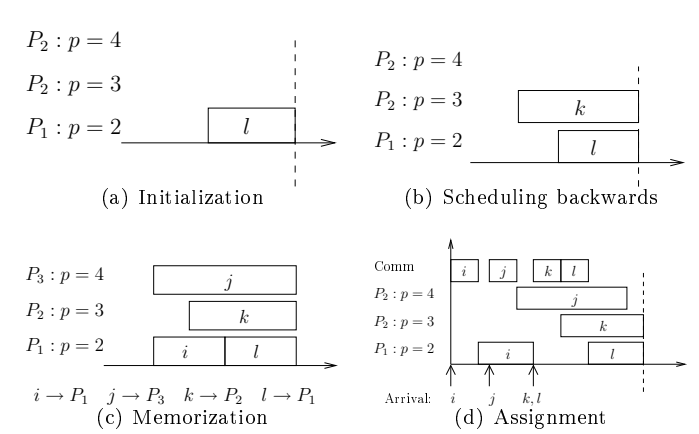
Figure 1. Different steps of the SLJF algorithm, with four tasks i , j , k , and l .
