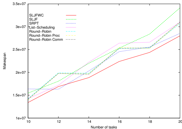
Figure 7. Makespan with release dates.
