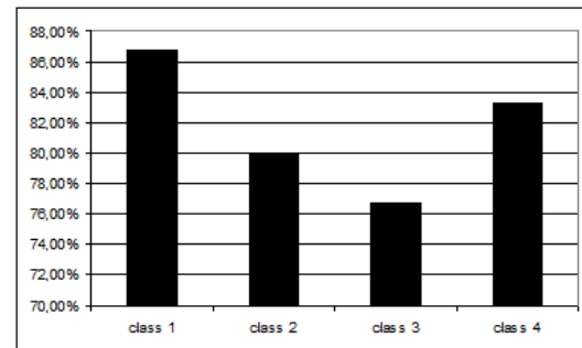
Figure 2. Classification rates for the 4 pose classes
