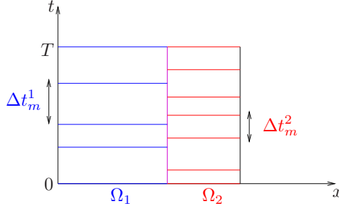
Figure 5.1: Nonconforming time grids in the subdomains.
