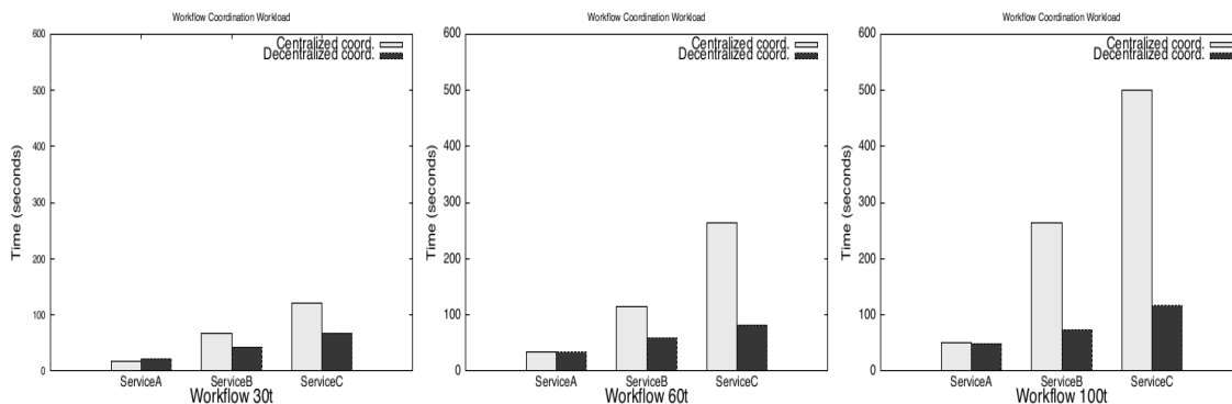
Figure 19: Coordination workload: centralized vs decentralized
