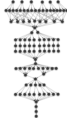
Figure 13: 100-task graph.
