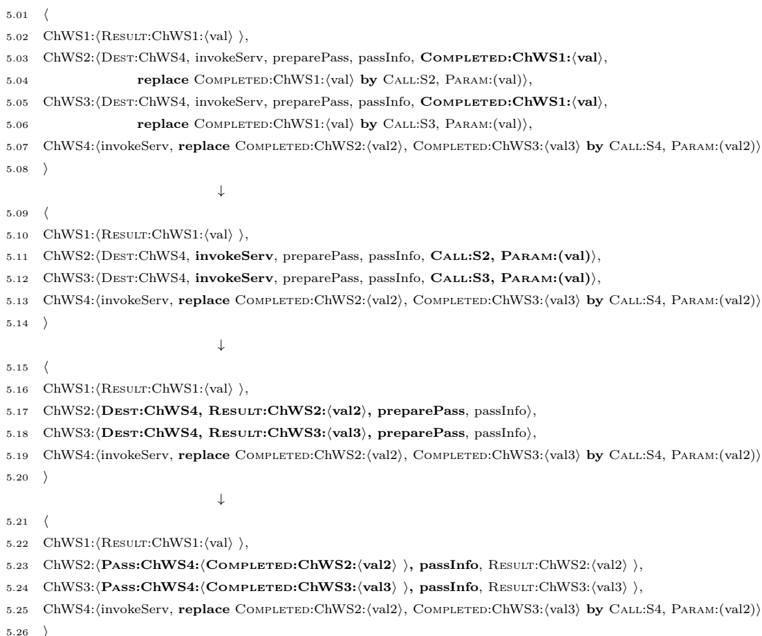
Figure 7: Workflow execution, steps 4-7.
