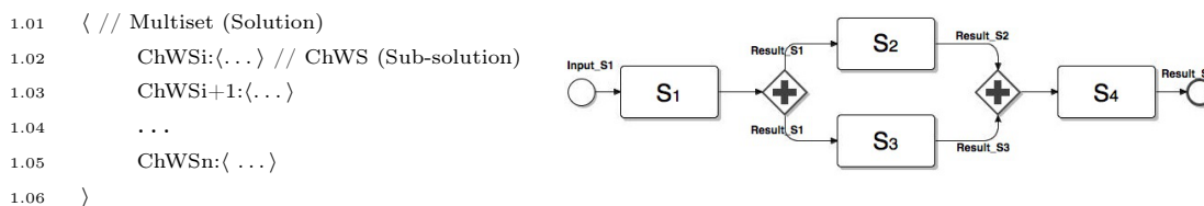
Figure 4: Chemical workflow representation (left), Simple workflow example (right).
