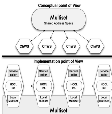
Figure 3: Points of view of the architecture.
