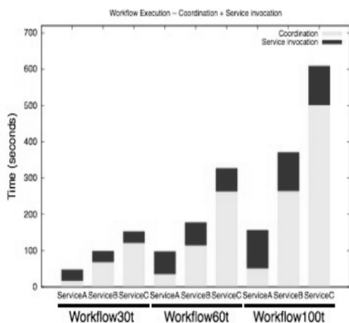
Figure 17: Centralized execution: ratio between coordination and invocation.
