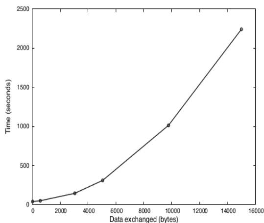
Figure 18: Performance results, data exchange.
