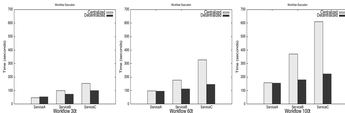
Figure 14: Workflow30t
