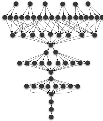
Figure 12: 60-task graph.
