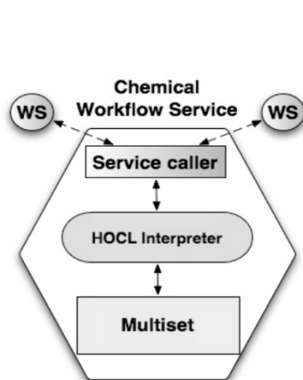
Figure 9: Centralized architecture.
