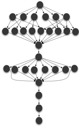
Figure 11: 30-task graph.
