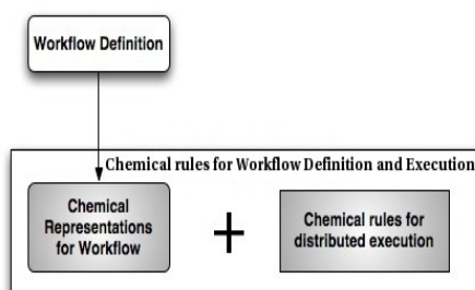
Figure 2: Chemical workflow.
