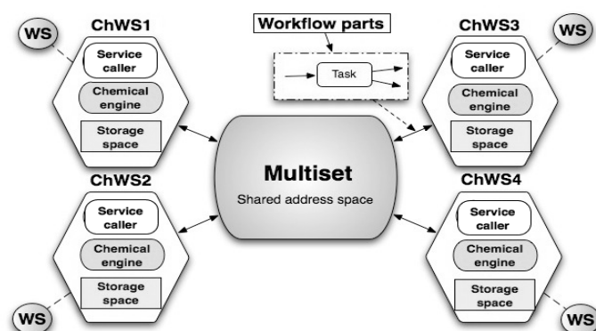
Figure 1: The proposed architecture.
