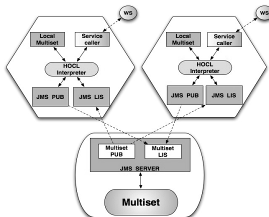
Figure 10: Decentralized architecture.
