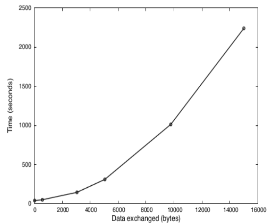
Figure 18: Performance results, data exchange.
