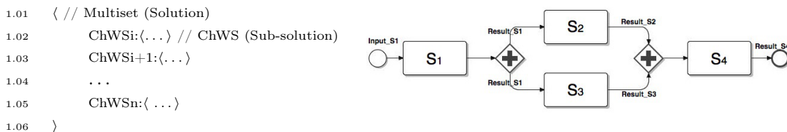
Figure 4: Chemical workflow representation (left), Simple workflow example (right).
