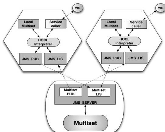
Figure 10: Decentralized architecture.
