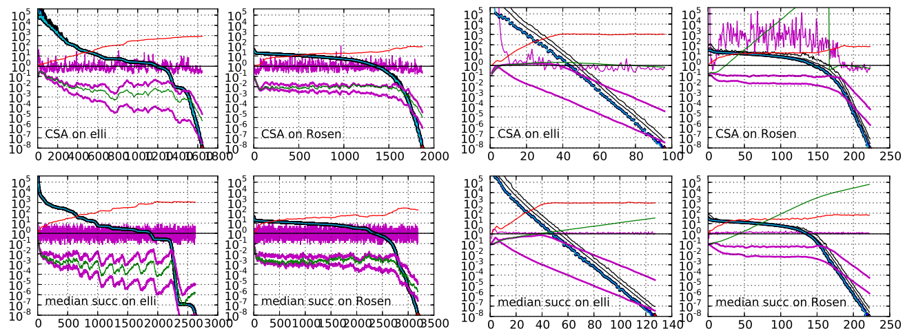
Figure 11: Single runs of the (\mu/\mu_w, \lambda) -ES on the ellipsoid and Rosenbrock function with \sigma_0 = 0.1 and on the Rosenbrock function \mathbf{x}_0 = (0.1, \dots, 0.1) , comparing cumulative step-size adaptation (CSA) with the median success rule (10)–(12), where the x -axis shows iterations. See Figure 4 for details.
