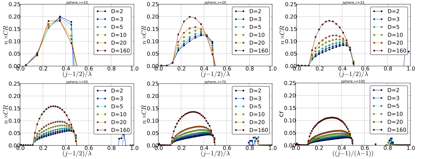
Figure 8: Normalized convergence rate at \hat{\sigma}_{1/2}(j) versus fitness comparison quantile, (j - 1/2)/\lambda , for different values of \lambda on the sphere function. \hat{\sigma}_{1/2}(j) being the step-size where the median success probability (LHS of (8)), given j , is the closest to 1/2 .
