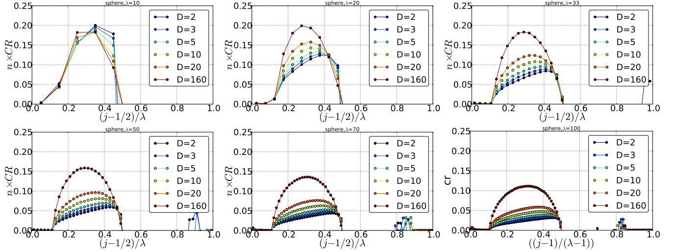
Figure 8: Normalized convergence rate at \hat{\sigma}_{1/2}(j) versus fitness comparison quantile, (j-1/2)/\lambda , for different values of \lambda on the sphere function. \hat{\sigma}_{1/2}(j) being the step-size where the median success probability (LHS of (8)), given j , is the closest to 1/2 .
